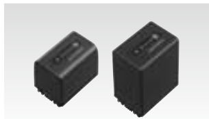
Rechargeable Battery Pack NP-FV70 (6.8 V / 14.0 Wh / 2060 mAh) NP-FV100 (6.8 V / 26.5 Wh / 3900 mAh)
